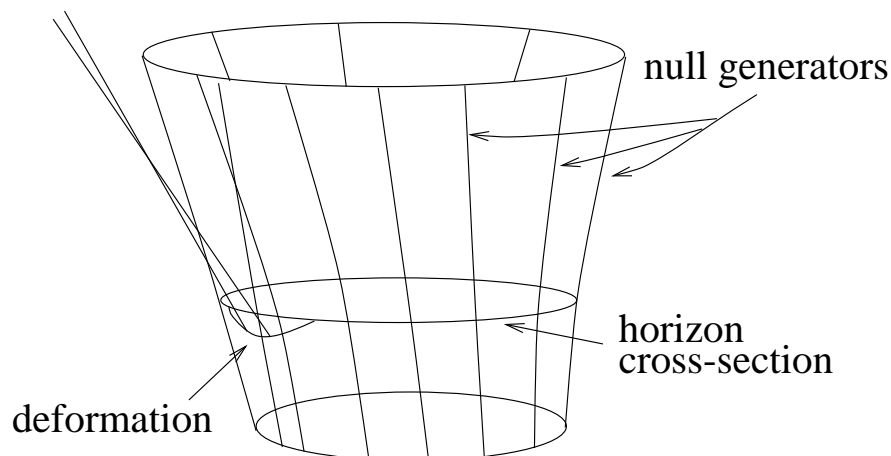
Figure 1.6: Portion of an event horizon with some converging generators that reach a crossing point. The generators of the boundary of the future of the deformation also reach a crossing point. The impossibility of this crossing point is used in proving the area theorem.
