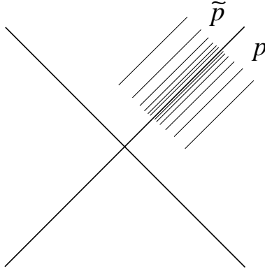
Figure 3.4: The mode p and its “flipped” partner \tilde{p} have both positive and negative u -frequency components, but the combination p + e^{-\pi\lambda}\tilde{p} has only positive frequencies.
