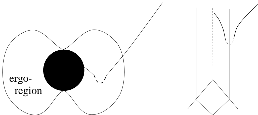
Figure 3.1: Pair production in the ergoregion of a rotating black hole (left); and Hawking effect: pair production straddling the horizon (right).
